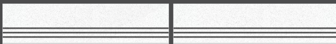
Quartz Crystal
